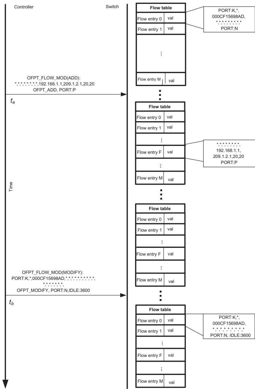
FIG. 5.8 Controller programming flow entries in V.1.0.
