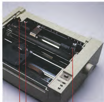
Sprocket Release Paper Clamps
